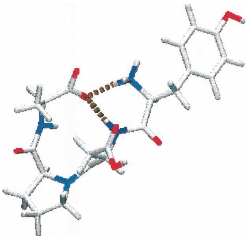
FIG. 1. Calculated conformation of H-Tyr-Asp-Pro-Ala-OH with H-bond between amino Tyr 1 and (or) Asp 2 and carboxyl Ala 4 groups (MOPAC 7.01).
